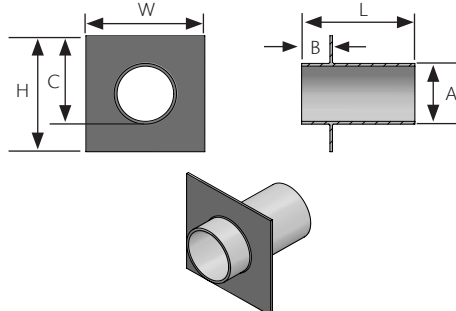
Pipe Connector with Flange
